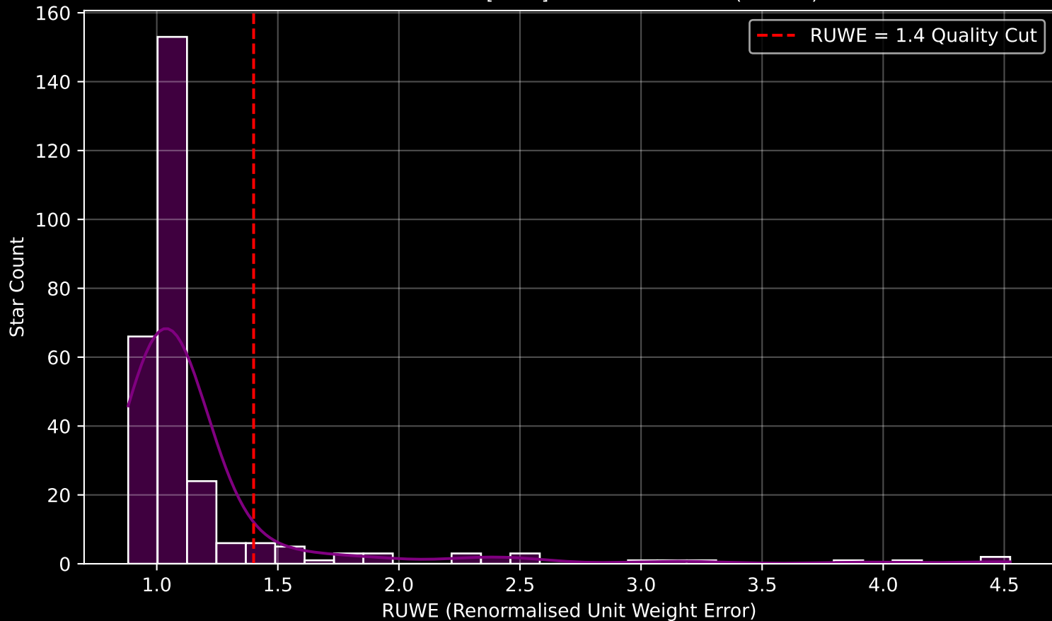
GALAH DR4 Field [6888] RUWE Distribution (n= 282)
