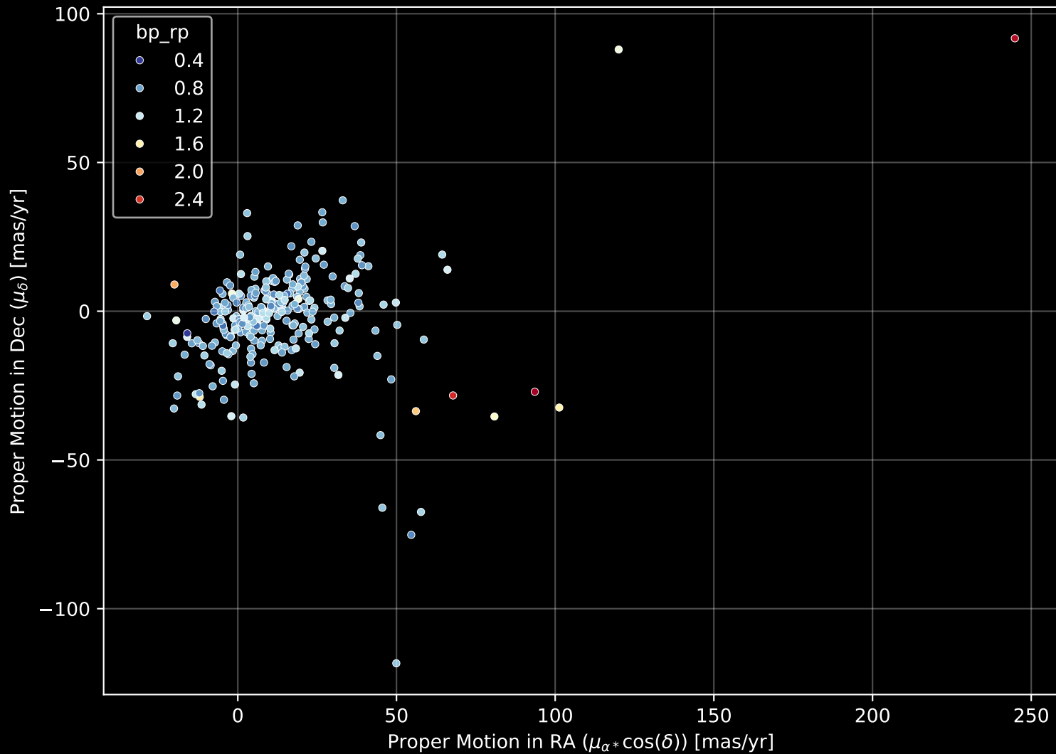
GALAH DR4 Field: [6888] Proper Motion Diagram (n= 288)
