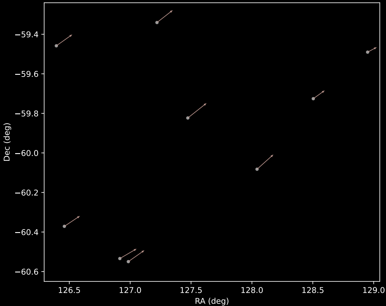
GALAH DR4 Cluster 11 Proper Motion Vectors (n=9)
