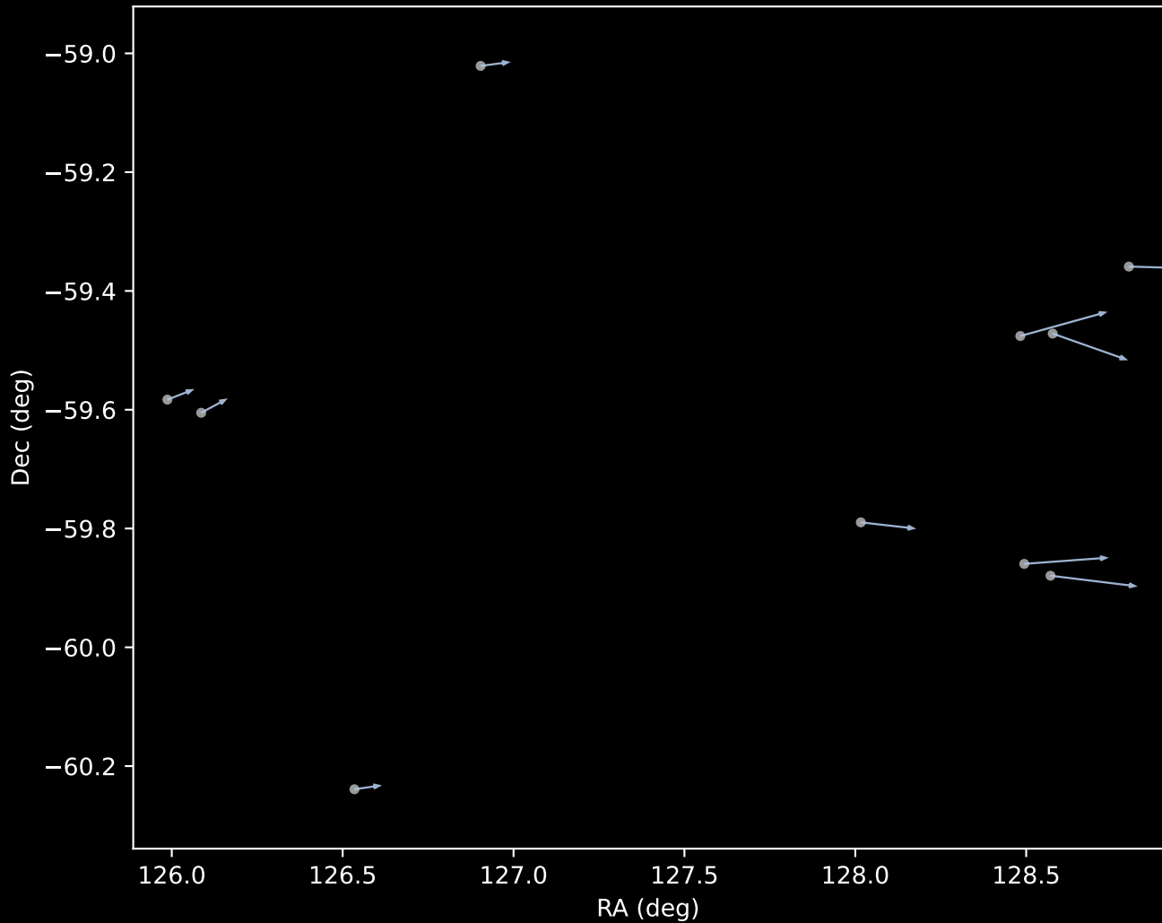
GALAH DR4 Cluster 1 Proper Motion Vectors (n=10)
