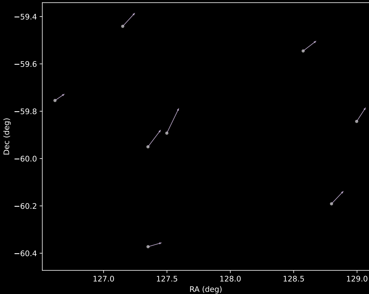
GALAH DR4 Cluster 9 Proper Motion Vectors (n=8)
