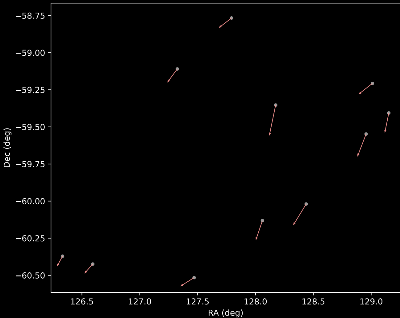
GALAH DR4 Cluster 7 Proper Motion Vectors (n=11)
