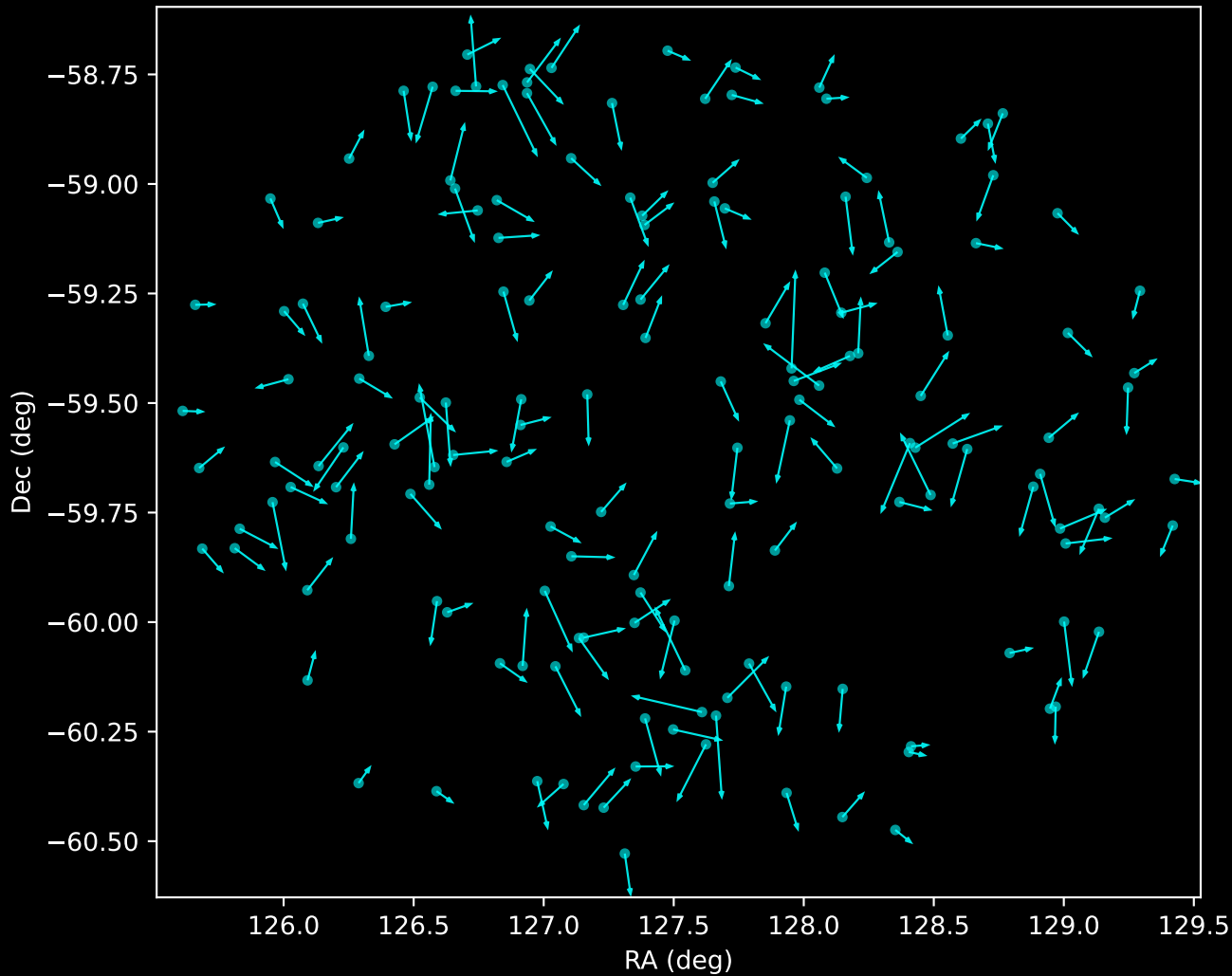
GALAH DR4 Noise Stream Proper Motion Vectors (n=159)
