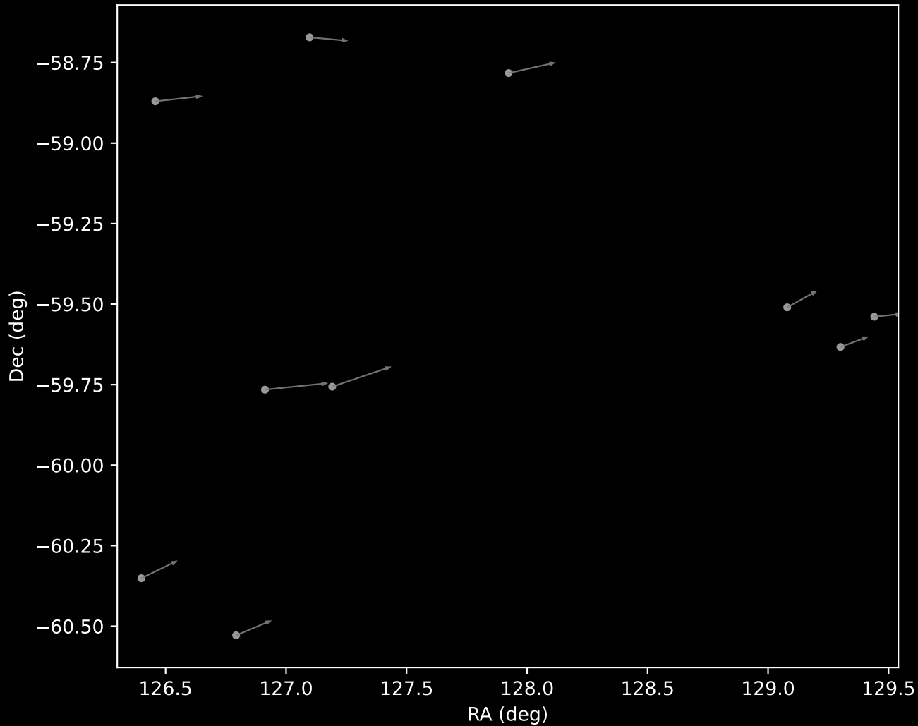
GALAH DR4 Cluster 14 Proper Motion Vectors (n=10)
