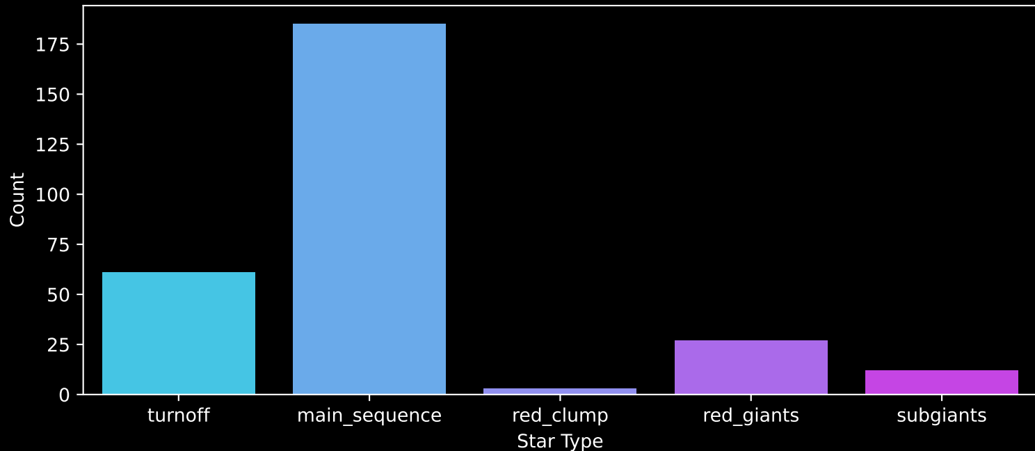
GALAH DR4 Field: [6888] Count plot of Star Type
